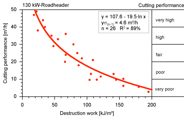
Figure 2. Roadheader cutting performance versus destruction work (slate and quartzite, Sewage tunnel Zeulenroda, Germany).
