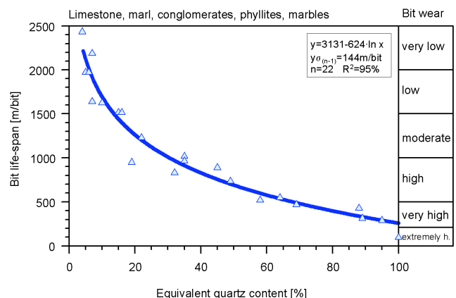
Figure 9. Drilling bit lifetime of rock types with grain-grain boundaries versus equivalent quartz content (8 tunnel projects).
