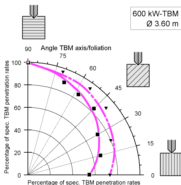
Figure 11. Mean values of specific TBM penetration rates in phyllite (full line) and phyllite – carbonate-schist interstratification (dashed line) versus angle of foliation. Schönberg pilot tunnel, Schwarzach, Austria.
