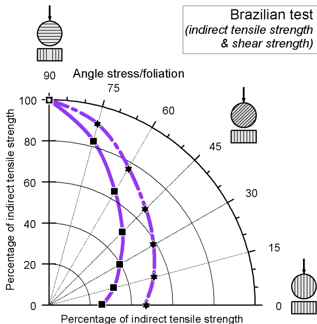
Figure 12. Mean values of Brazilian test results in two different quartzphyllites versus angle of foliation. Inntal tunnel, Innsbruck, Austria.
