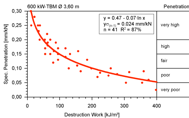
Figure 4. Specific TBM penetration rates versus destruction work (phyllite & carbonate schist, Schönberg pilot tunnel, Schwarzach, Austria).
